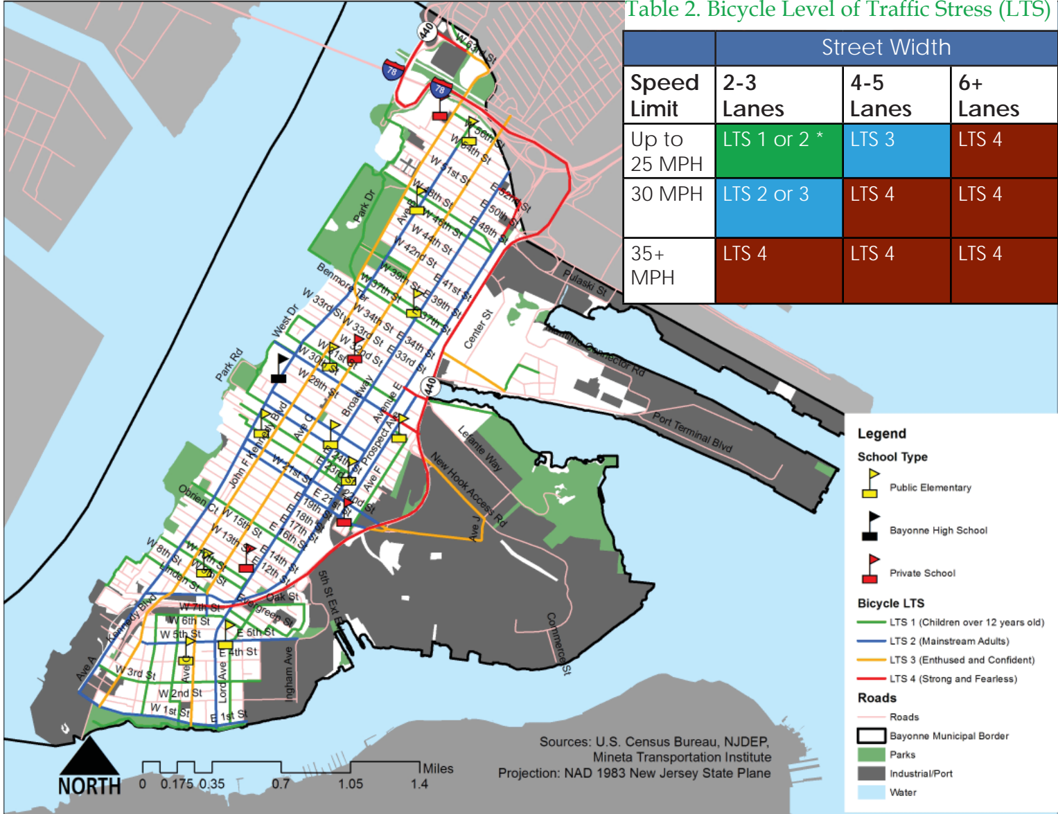
Figure 13. Bicycle Level of Traffic Stress map
