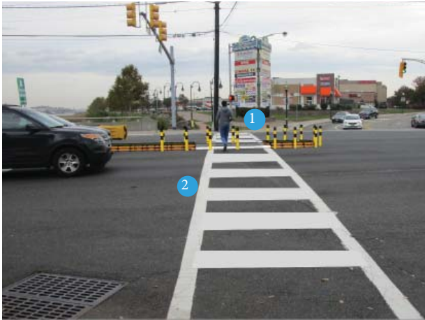
Figure 37. After: More visible crosswalks and a pedestrian refuge
