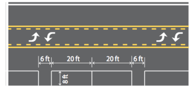
Figure 39. Paired parking
