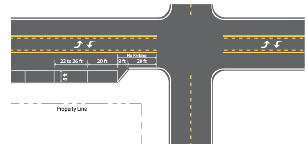
Figure 40. Parking lane transition
